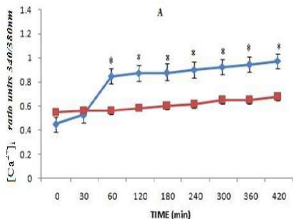
Figure 1: Time-course changes in [\text{Ca}^{2+}]_i expressed as fluorescence ratio units (intensity) in Fura-2 AM loaded 1321N1 cell lines
