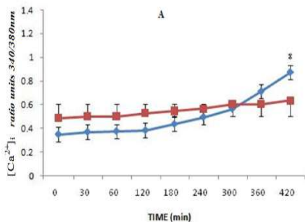
Figure 2: Time-course changes in [\text{Ca}^{2+}]_i expressed as fluorescence ratio units (intensity) in Fura-2 AM loaded Gos-3 cell lines.
